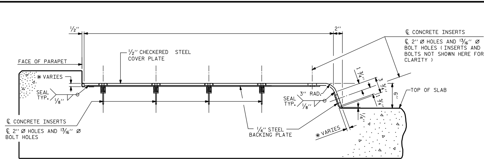
END VIEW (NORMAL TO SIDEWALK)
