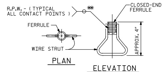
CONCRETE INSERT
